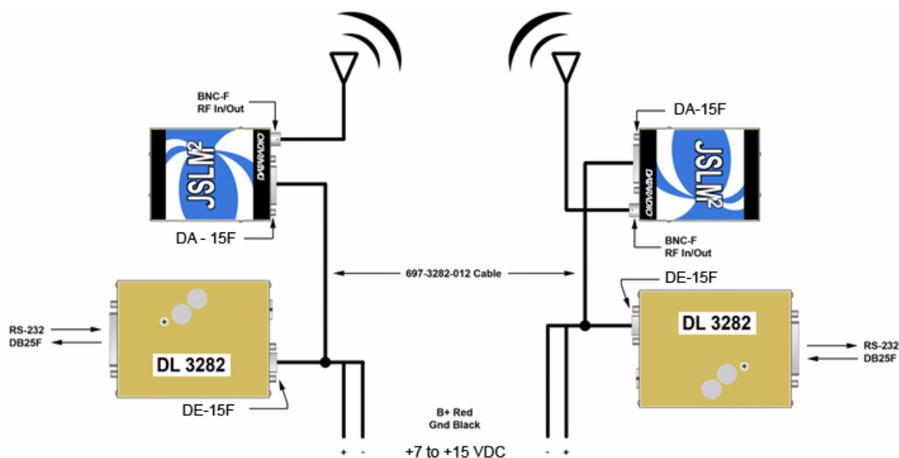
Figure 1 Typical JSLM2 - Modem Configuration Connection
