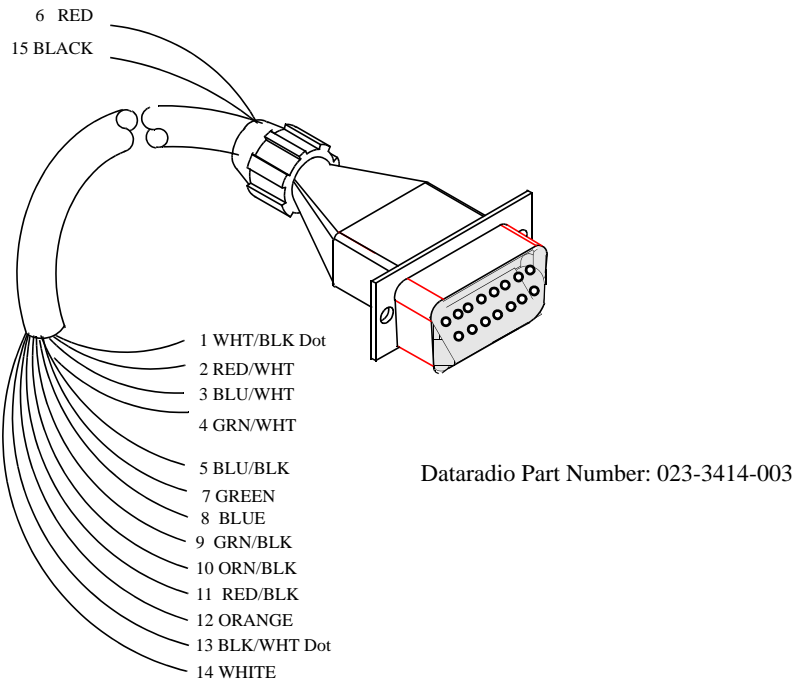
Figure 2-2 JSLM2 Accessory Interconnect Power Cable
