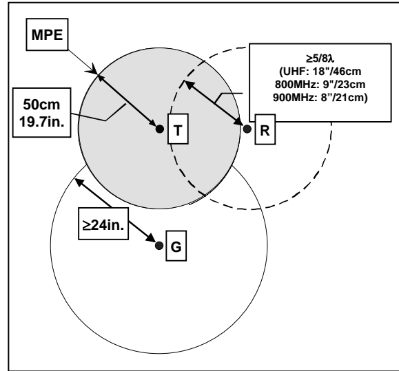
Figure 4 - Antenna spacing
