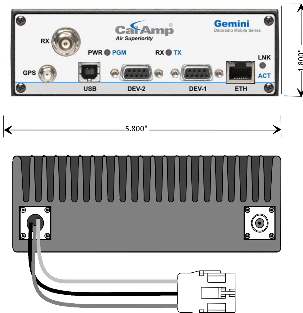
Figure 6 - Front and rear panels
