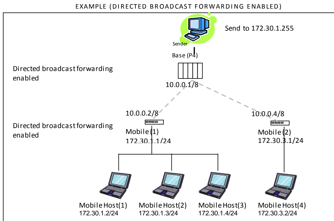
Figure 33 - Example of Directed broadcast forwarding enabled
