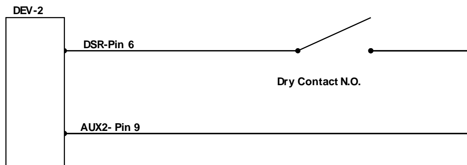
Figure 57 - Appendix 1 – Alarm Function, Dry Contact Connection
