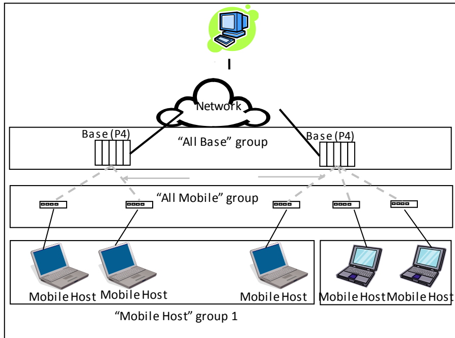
Figure 39 - Typical E-DBA Multicast Groups
