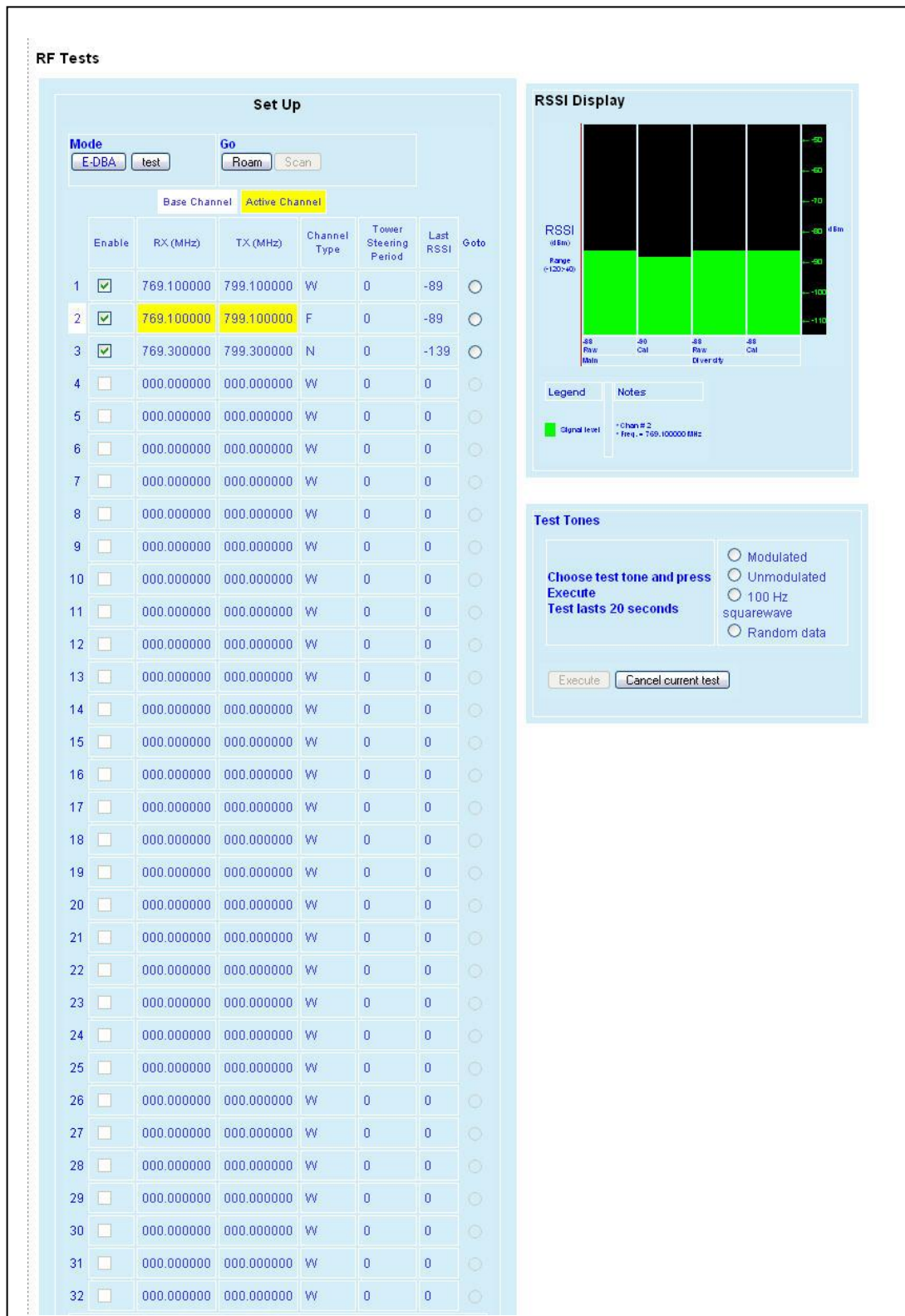
Figure 53 - Control - RF Tests
