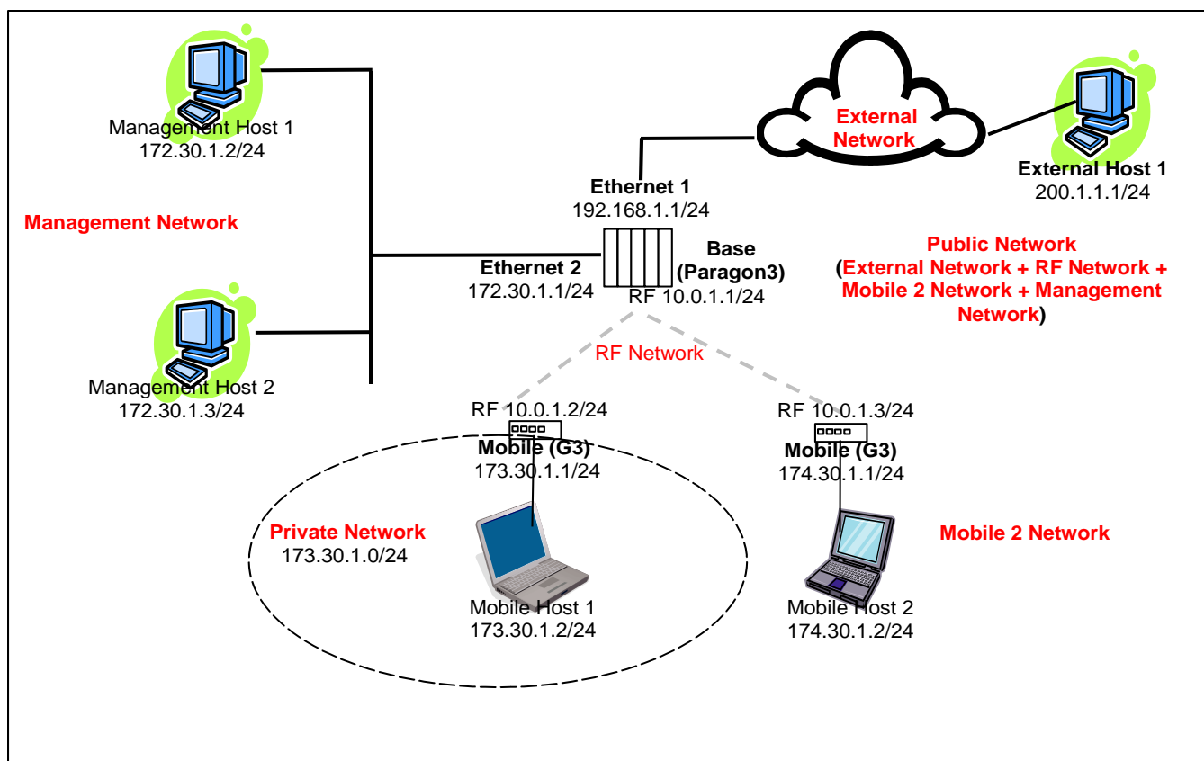
Figure 25 - Paragon4 - Private to Public Network (RF)
