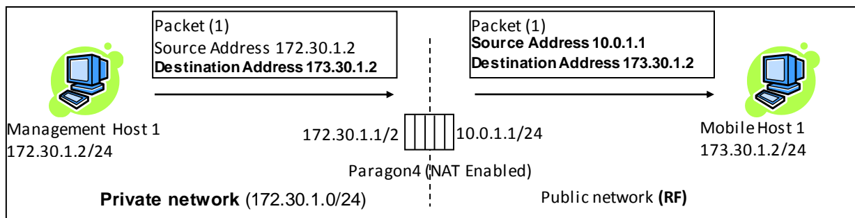
Figure 26 - NAT Enabled on GeminiG3
