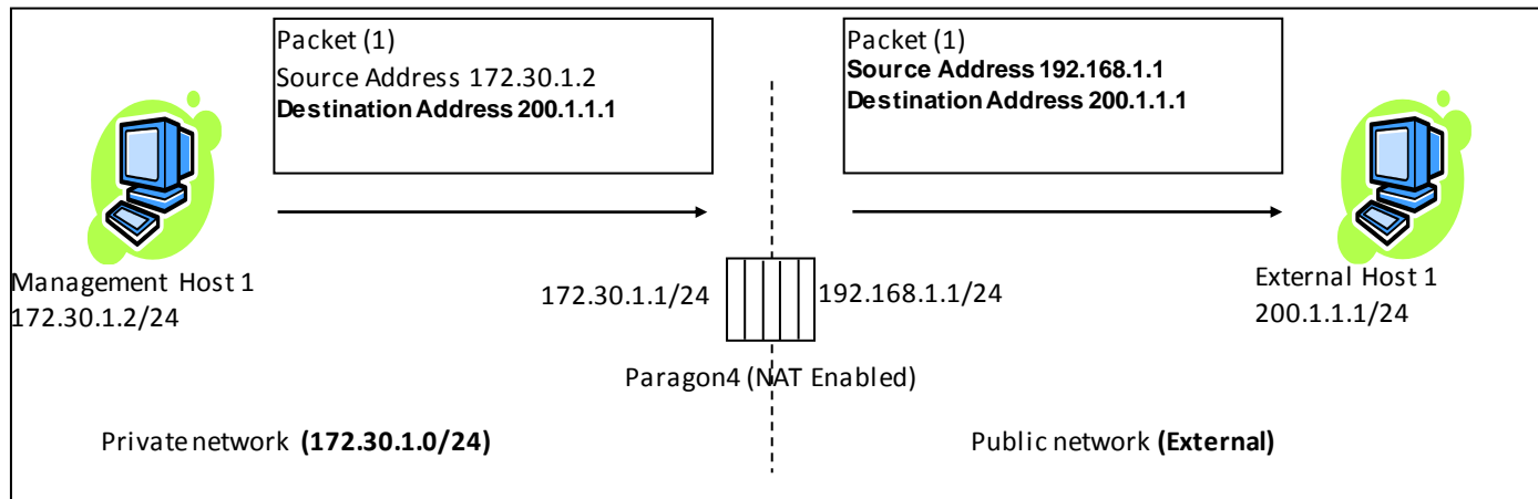
Figure 24 - Private to Public(External)
