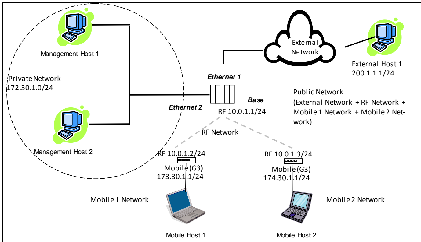
Figure 23 - NAT Enabled on Paragon4
