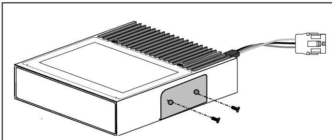
Figure 2 - Bracket installation
