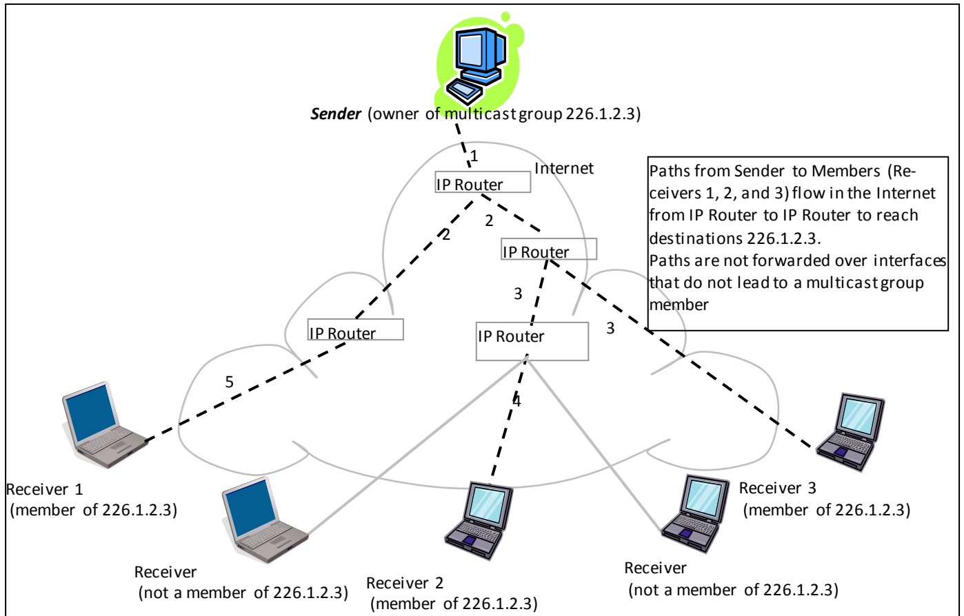
Figure 38 - Reception of multicast packets (Second step)
