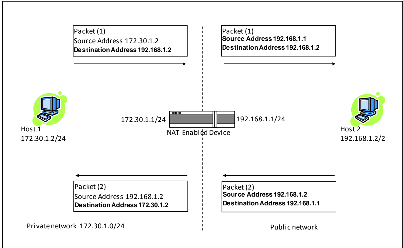
Figure 22 - Basic NAT Operations
