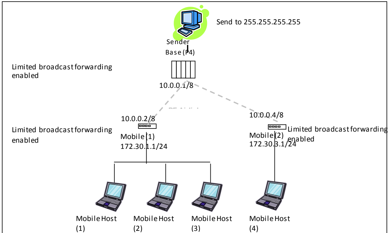
Figure 35 - Example of Directed broadcast forwarding enabled
